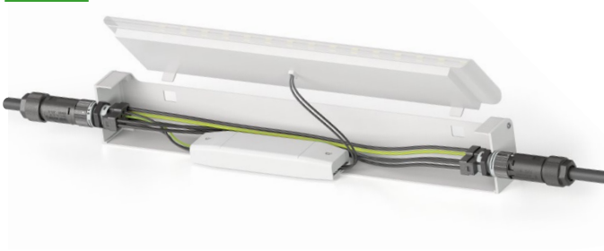
EXAMPLE THROUGH-WIRING 5-POLE
